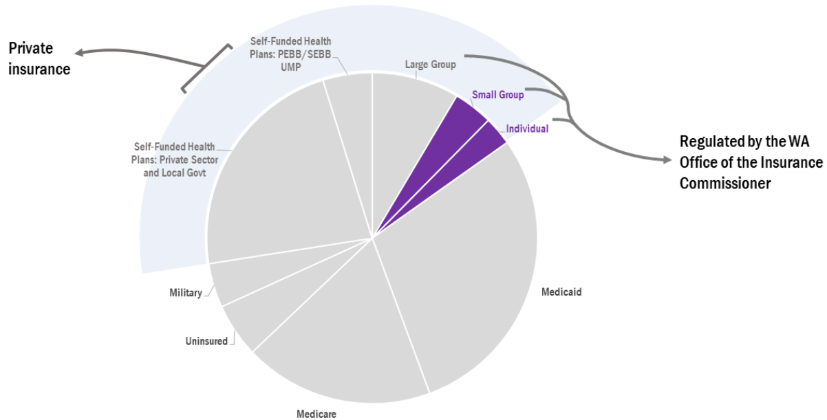
Source of Health Coverage for Washington Residents 2022 Impacted by the Reinsurance Policy Option
